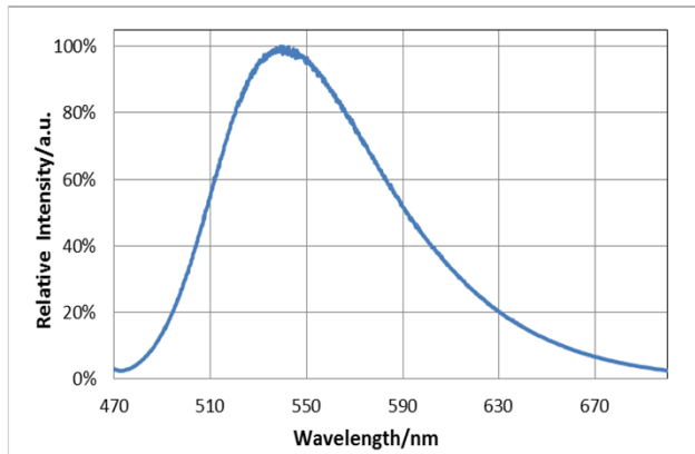
Emission Spectrum
