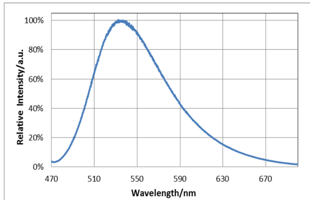
Emission Spectrum
