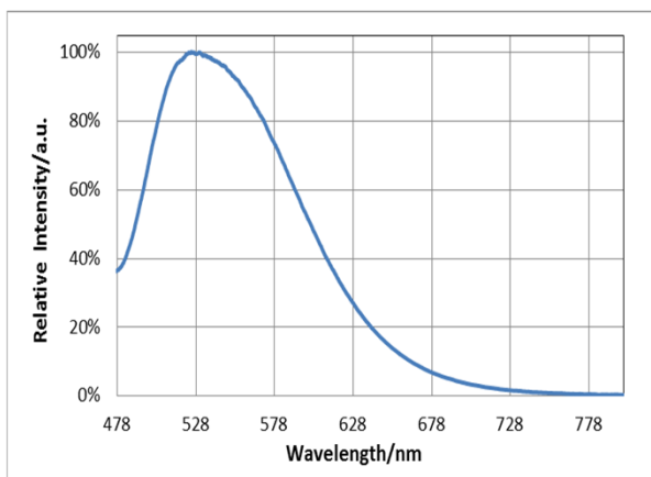
Emission Spectrum
