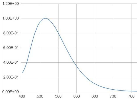
Emission Spectrum
