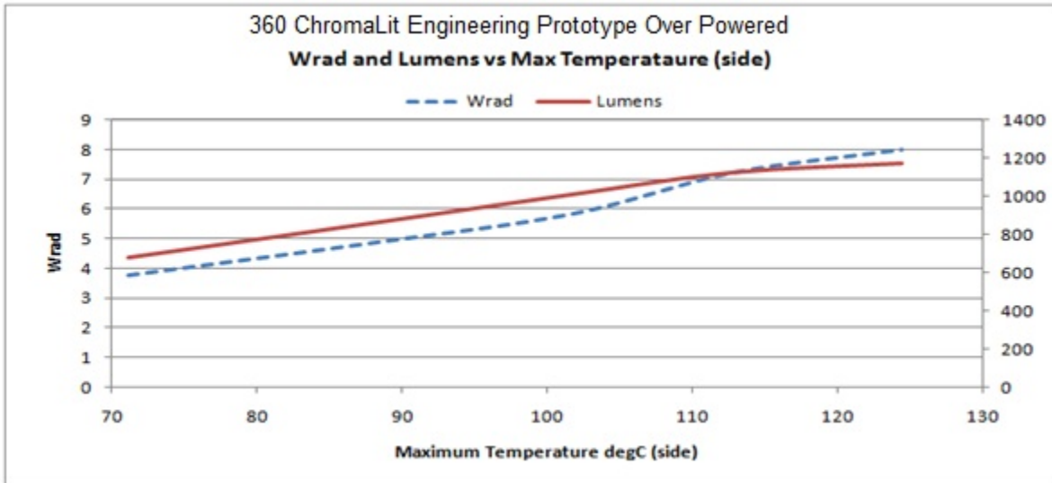
Fig 15. Over Powered Engineering Prototype, Lumens and Wrad
