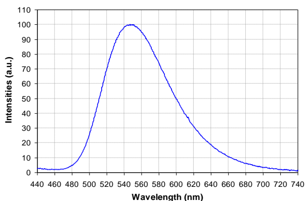
Emission Spectrum
