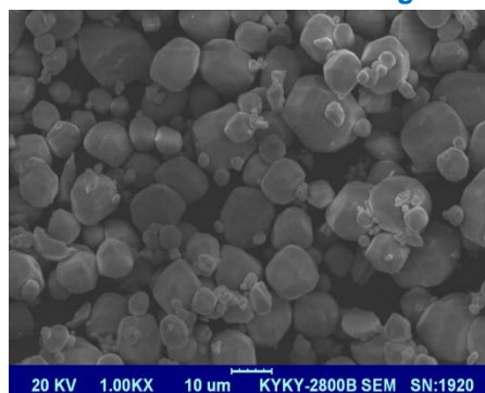
Particle Size: SEM Image
