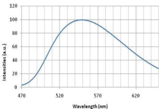
Emission Spectrum
