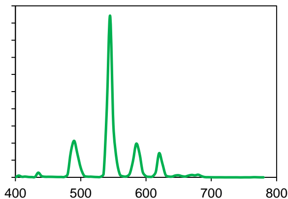
Emission Spectrum
