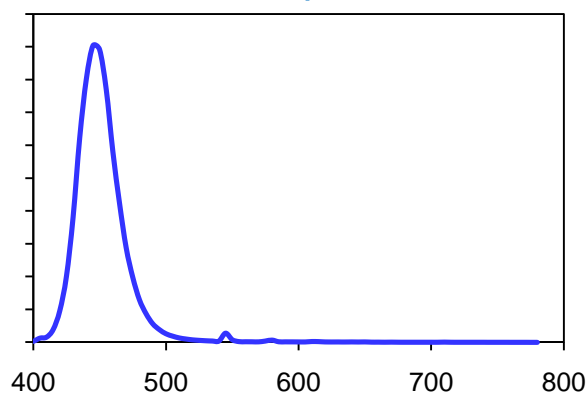
Emission Spectrum
