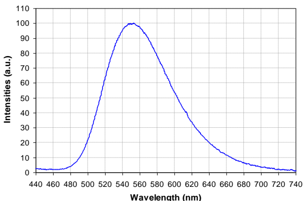
Emission Spectrum
